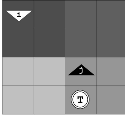
Figure 5.5: UAV Reconnaissance problem, in a grid of 4 x 4 sectors.
